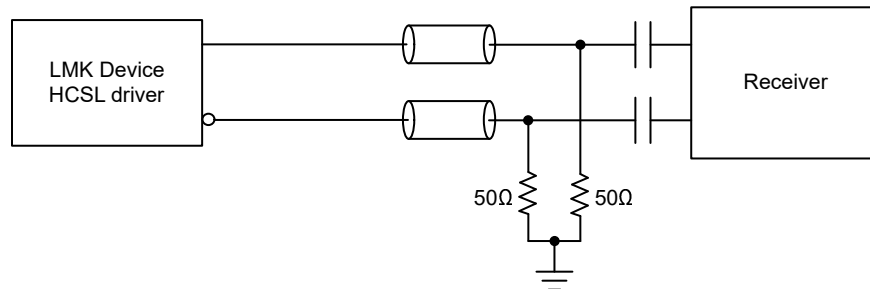
図 8-31. AC-Coupled HCSSL Output Termination
