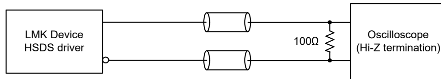
図 7-5. HSDS Output Time Domain Test Configuration
