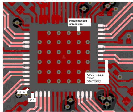
図 9-5. PCB Layout Example for LMK5C33414AS1, Top Layer
