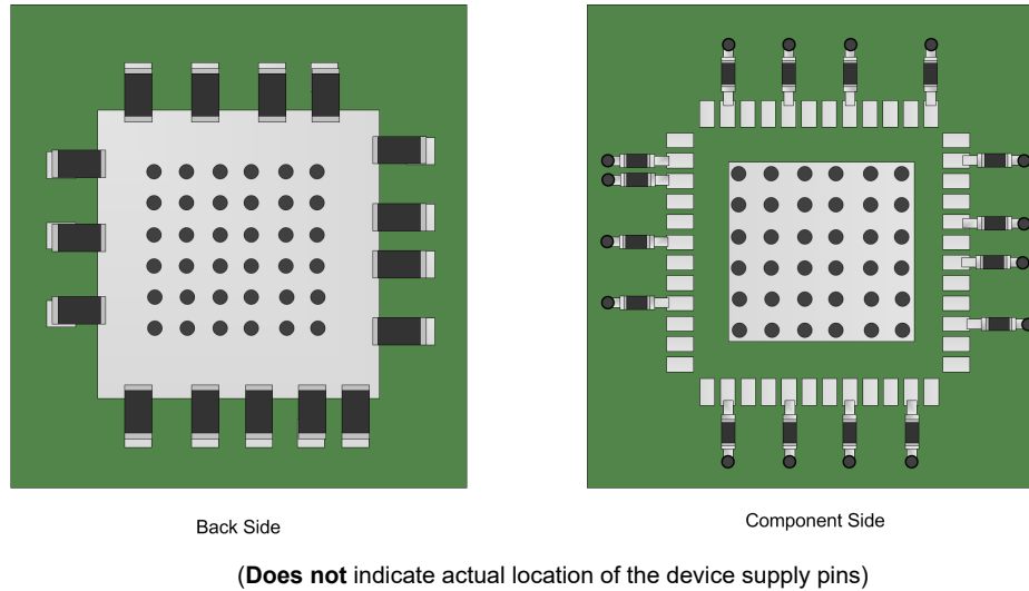
図 9-4. Generalized Placement of Power Supply Bypass Capacitors
