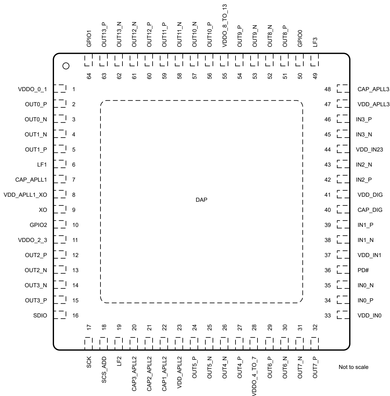
図 5-1. LMK5C33414AS1 RGC Package 64-Pin VQFN Top View
