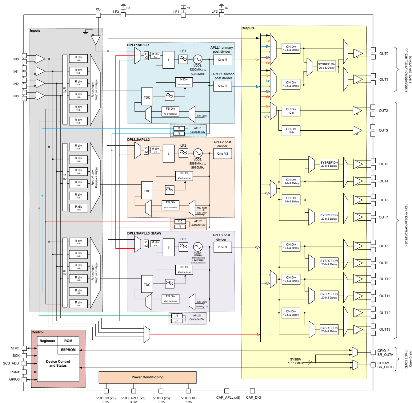
図 8-1. LMK5C33414AS1 Top-Level Block Diagram
