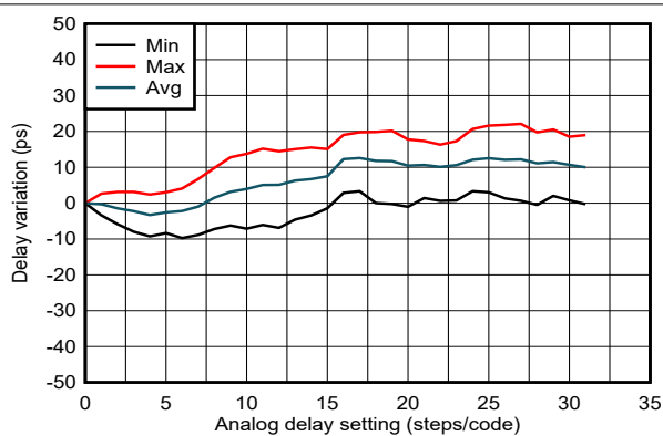
6-23. SYSREF/1PPS Delay Linearity vs. Analog Delay Code 5
