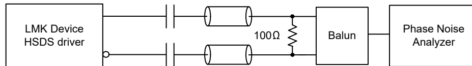
図 7-6. HSDS Output Phase Domain Test Configuration
