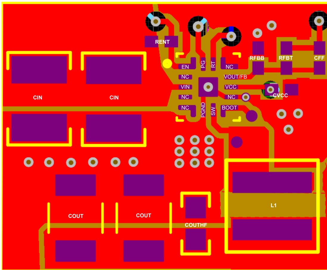
9-13. Example Layout
