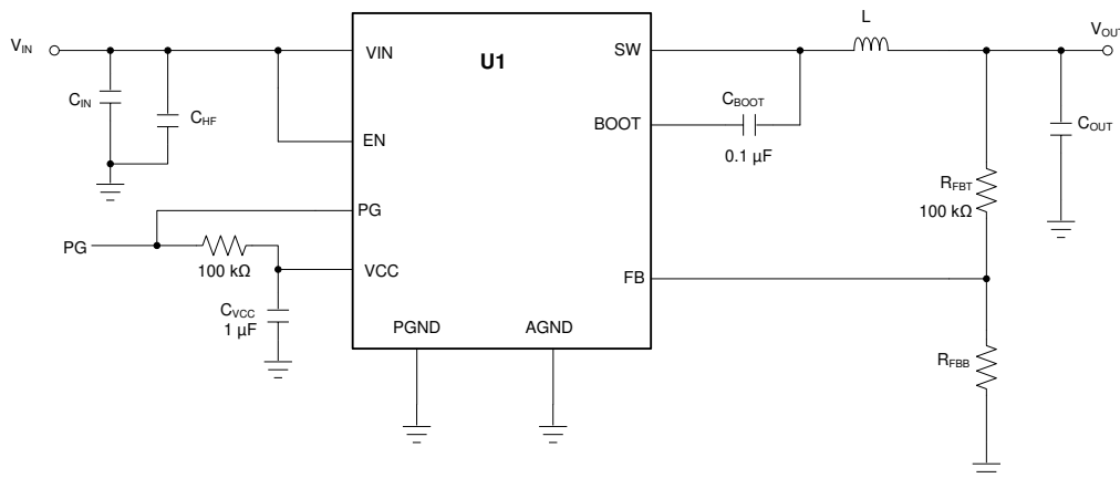
FIG 36. Circuit for Application Curves
