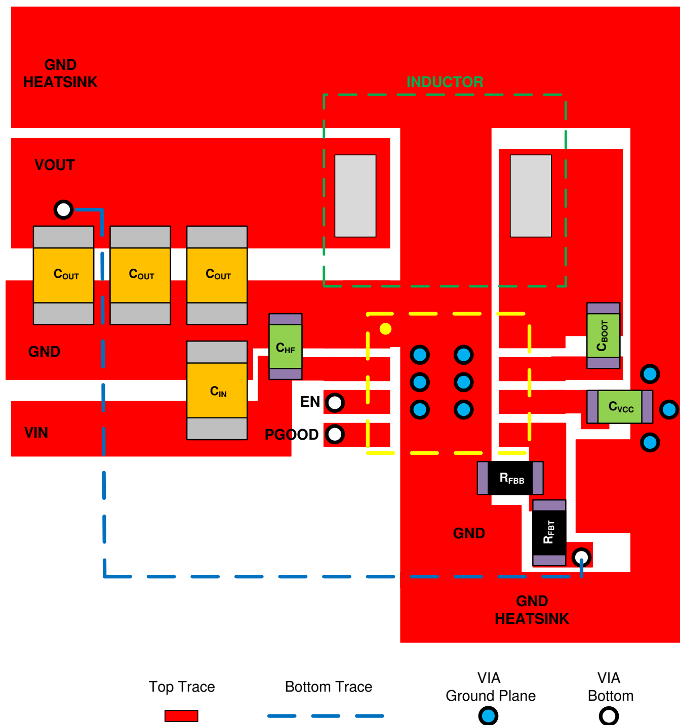
38. Example Layout for HSOIC (DDA) Package
