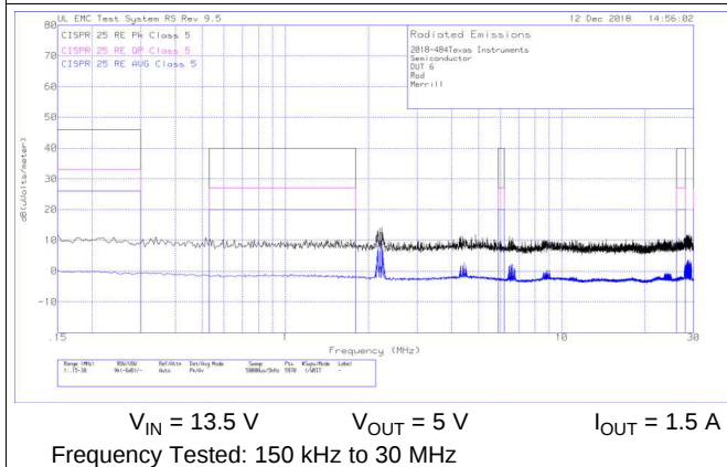
図 38. Radiated EMI Rod vs. CISPR25 Limits
