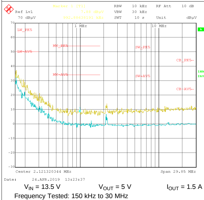
図 36. Conducted EMI vs. CISPR25 Limits (Yellow: Peak Signal, Blue: Average Signal)
