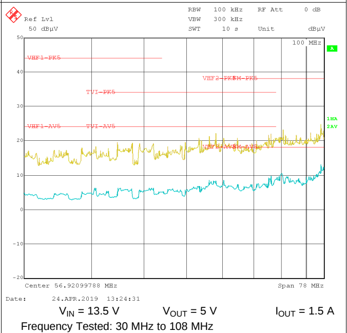
図 37. Conducted EMI vs. CISPR25 Limits (Yellow: Peak Signal, Blue: Average Signal)
