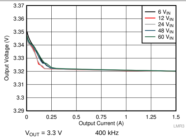
Figure 25. Load Regulation
