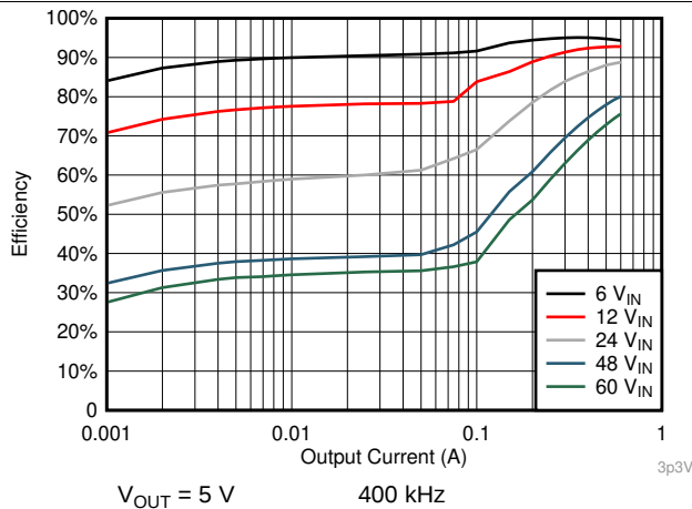
Figure 22. Efficiency
