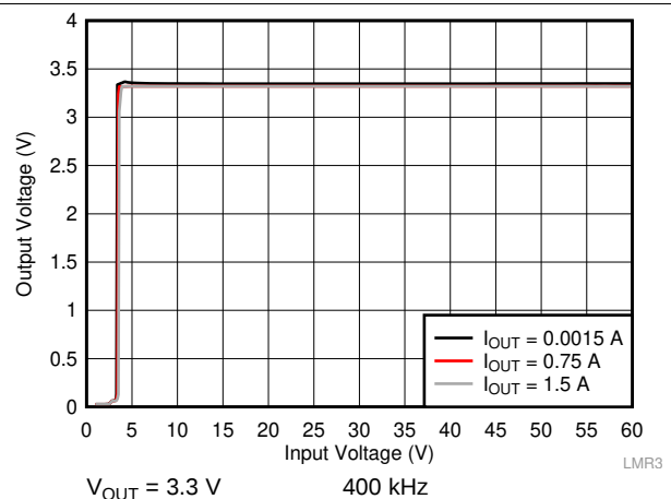
Figure 27. Line Regulation
