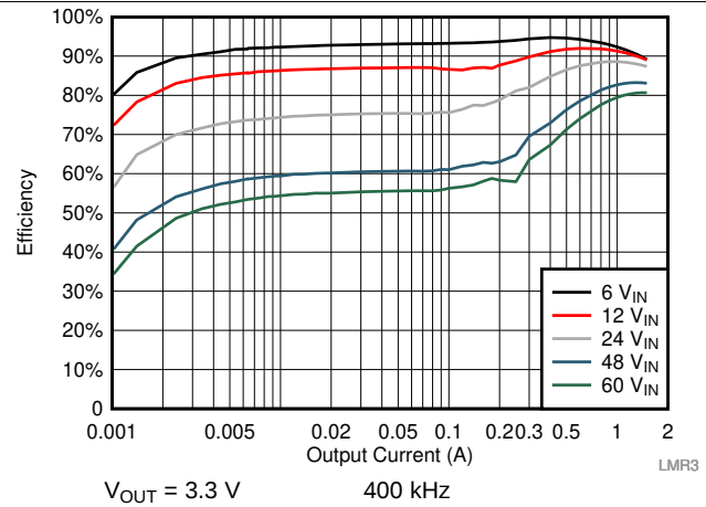
Figure 23. Efficiency
