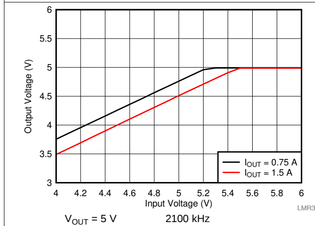
Figure 48. Overall Dropout Characteristic
