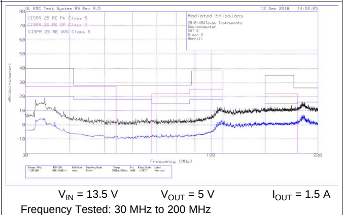
図 39. Radiated EMI Bicon Vertical vs. CISPR25 Limits
