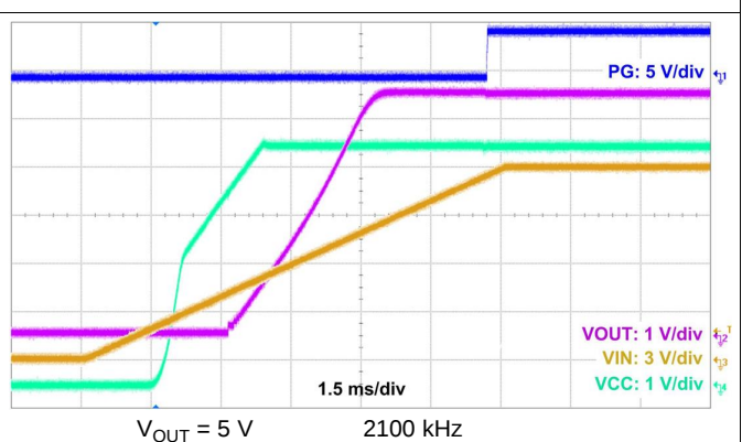
Figure 51. Start-Up Waveform
