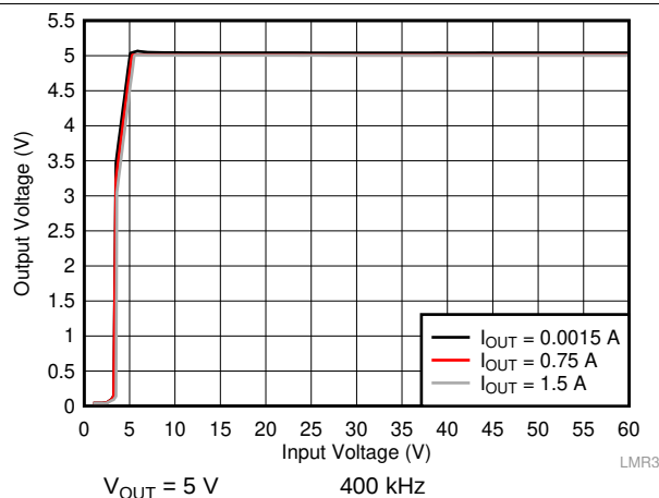
Figure 26. Line Regulation
