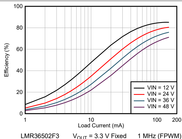
Figure 7-1. Efficiency
