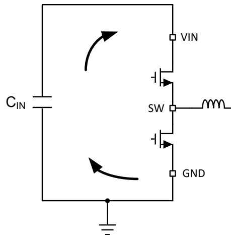
☒ 9-15. Current Loops with Fast Edges
