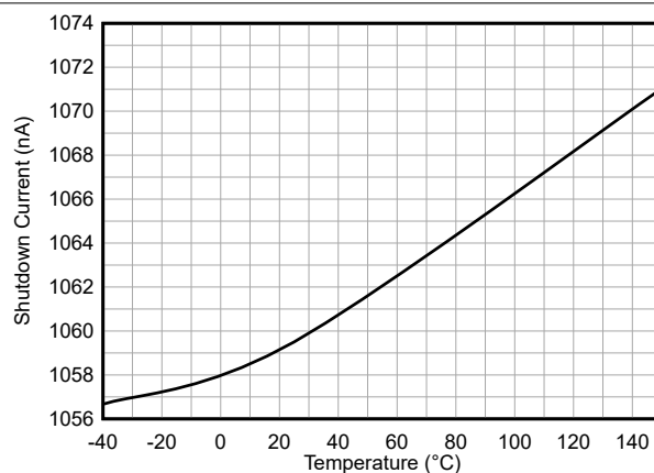
Figure 7-2. Typical Shutdown Current for 24-V VIN
