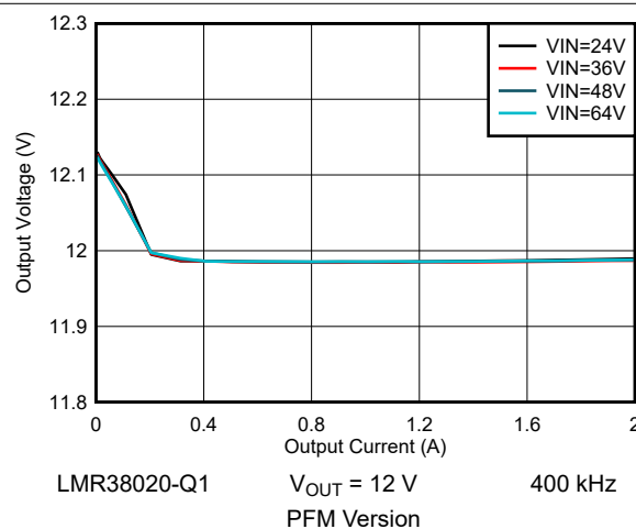
8-14. 12-V Load Regulation
