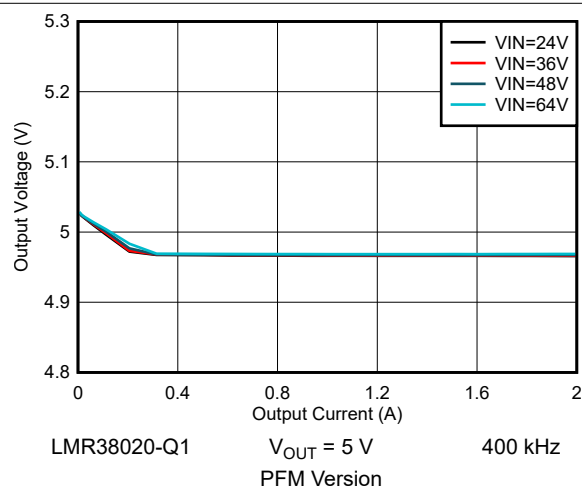
8-13. 5-V Load Regulation
