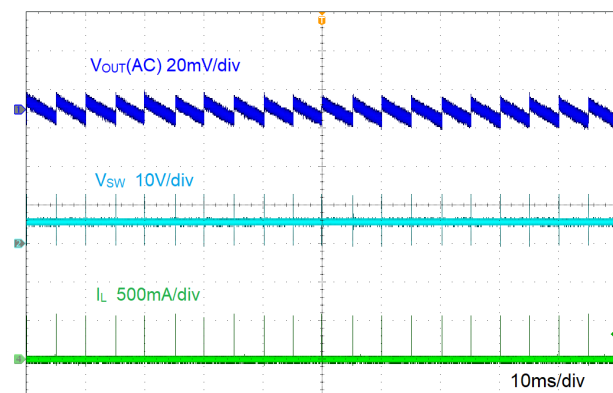
图 8-2. Ripple at No Load
