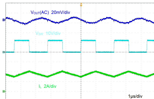
图 8-3. Ripple at Full Load
