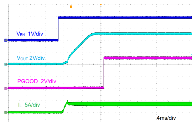
图 8-5. Start-Up by EN
