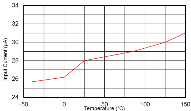
Figure 6-13. Non-Switching Input Supply Current
