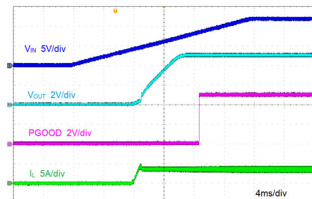
图 8-4. Start-Up by V_{IN}
