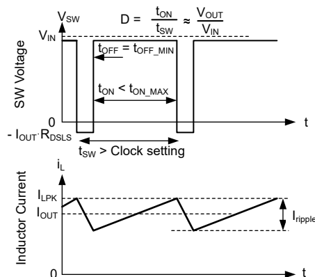
図 7-10. Dropout Waveforms
