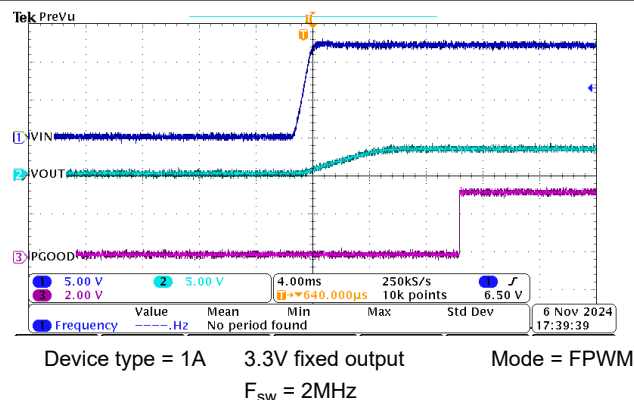
8-5. Start-up
