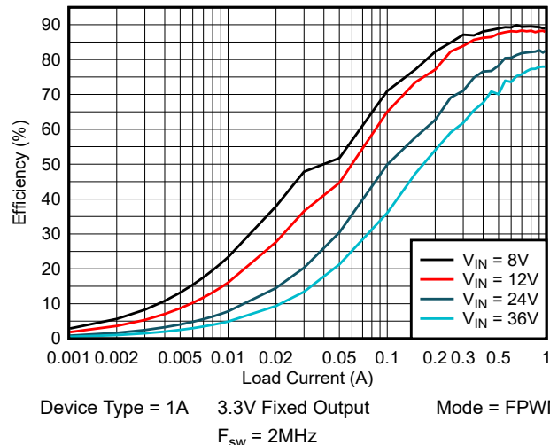
8-2. Efficiency
