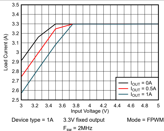
8-4. Dropout Voltage
