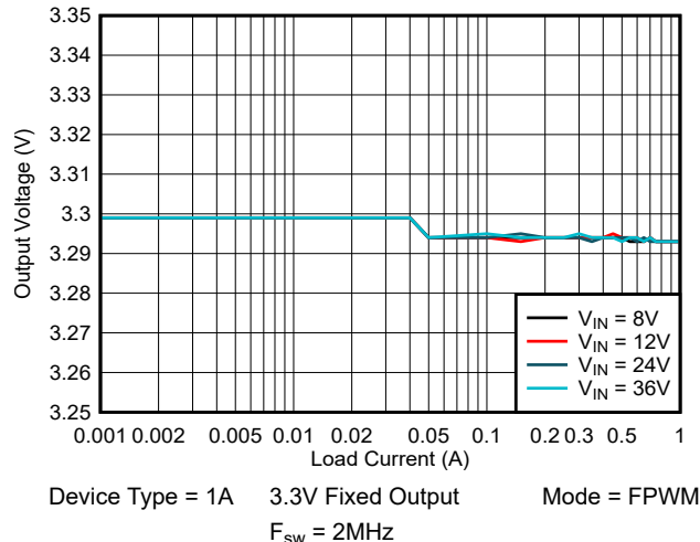
8-3. Load Regulation
