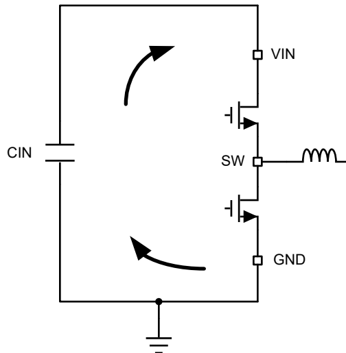
図 8-12. Current Loops With Fast Transients
