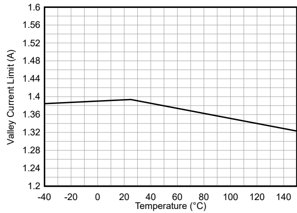
図 6-2. Valley Current Limit vs Temperature
