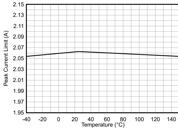
図 6-1. Peak Current Limit vs Temperature
