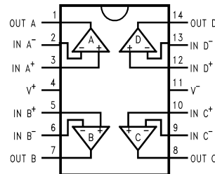
Pin Functions: LMV651
