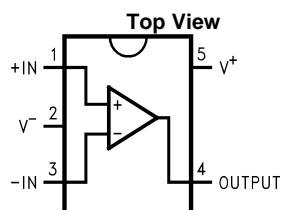
Figure 2. 5-Pin SC70 Package See Package Number DCK0005A
