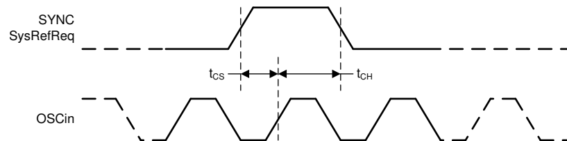
✎ 2. Trigger Signals Timing Diagram
