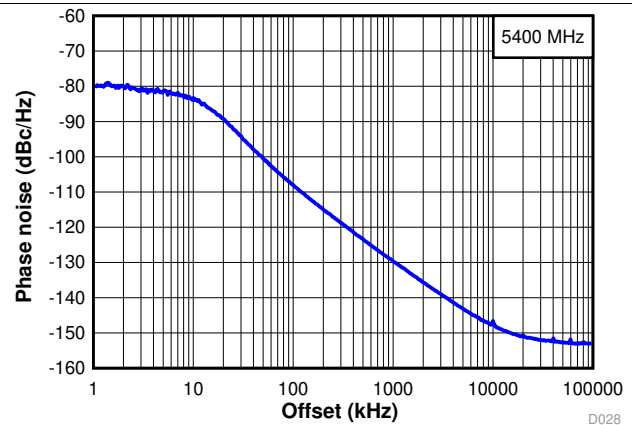
FIG 18. Narrow Band Phase Noise at 5.4 GHz
