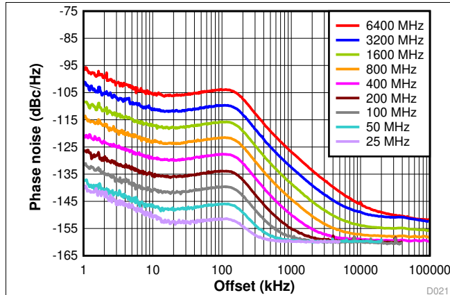
FIG 21. Direct and Divided Down Outputs
