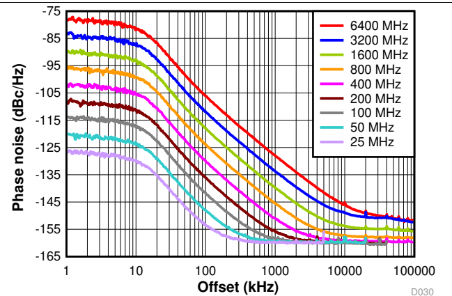
FIG 22. Direct and Divided Down Outputs
