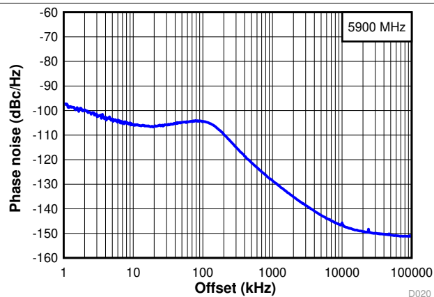
FIG 19. Wide Band Phase Noise at 5.9 GHz
