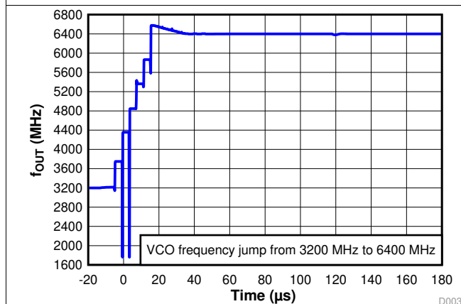
FIG 25. VCO Calibration Time
