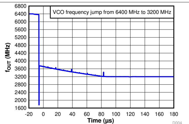
FIG 26. VCO Calibration Time
