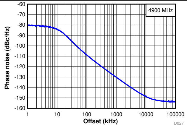
FIG 16. Narrow Band Phase Noise at 4.9 GHz
