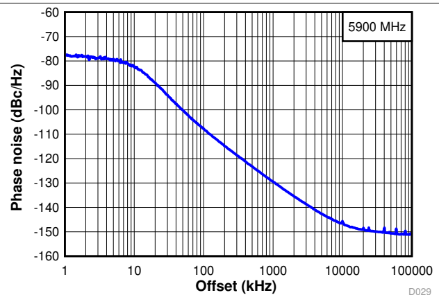
FIG 20. Narrow Band Phase Noise at 5.9 GHz
