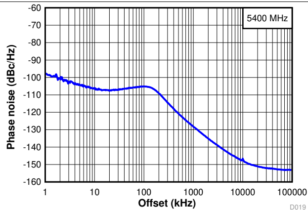
FIG 17. Wide Band Phase Noise at 5.4 GHz
