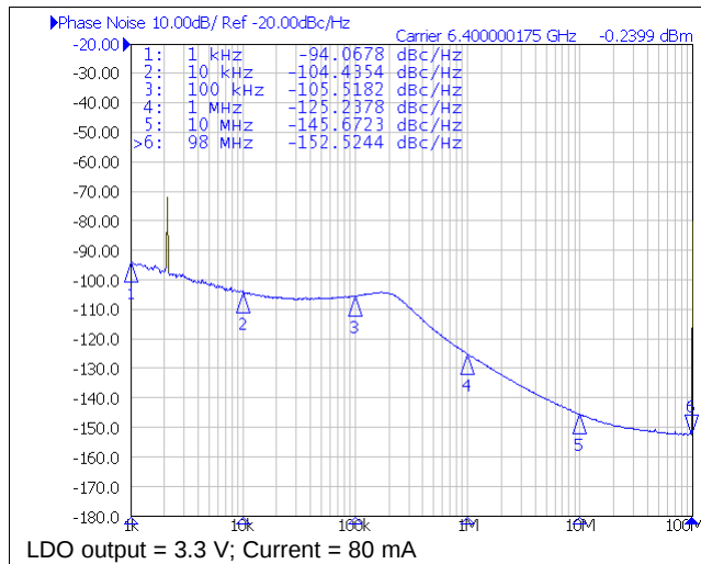
Figure 187. Phase Noise With LDO Power Supply
