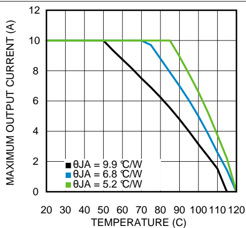
Figure 31. Thermal Derating
