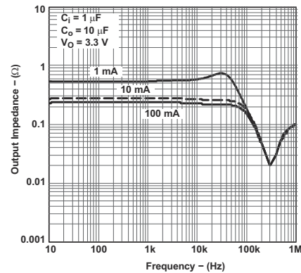
5-26. Output Impedance vs Frequency for Legacy Chip
