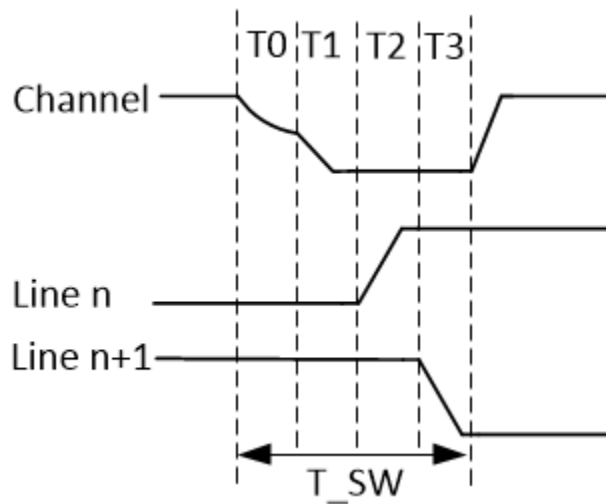
FIG 7-7. Line Transitioning Sequence
