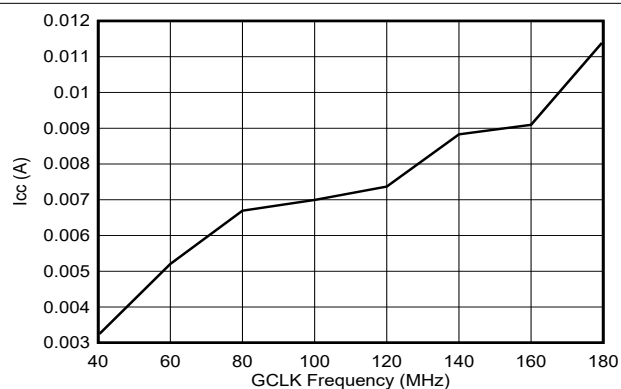
FIG 6-7. I CC Current vs GCLK Frequency
