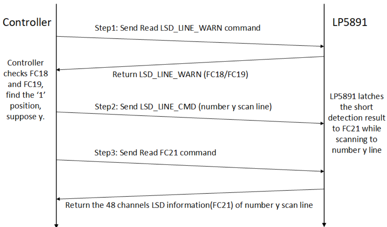
☒ 7-14. Steps to Read LED Short Information
