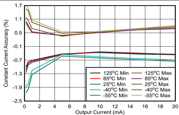
FIG 6-5. Channel to Channel Accuracy vs Output Current
