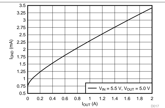
Figure 2. Ground Current vs Output Current
