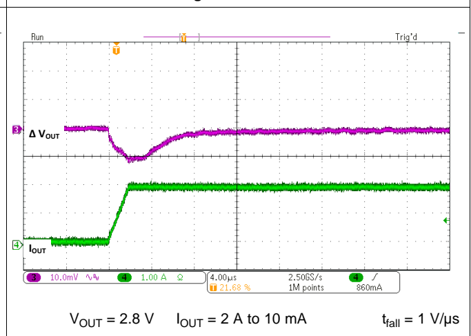
Figure 10. Load Transient Response
