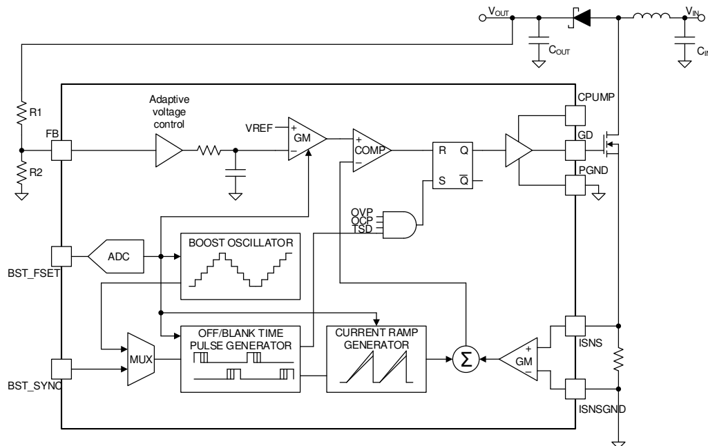
Figure 7-3. Boost Controller Block Diagram
