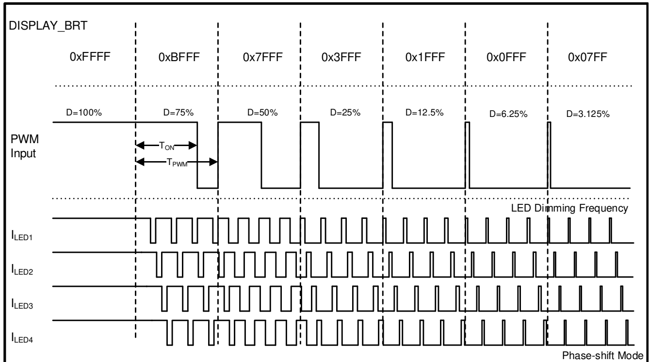
7-10. Phase-shift Dimming Diagram
