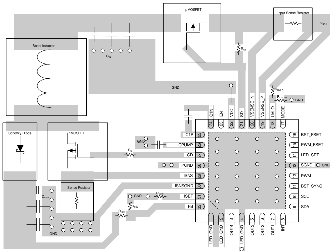
10-1. LP8864-Q1 Layout Guidelines
