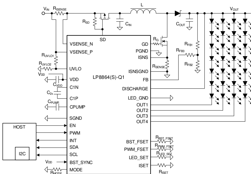
8-1. Full Feature Application for Display Backlight
