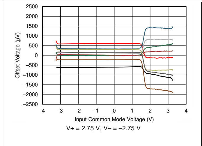
图 2. Offset Voltage vs Common-Mode Voltage
