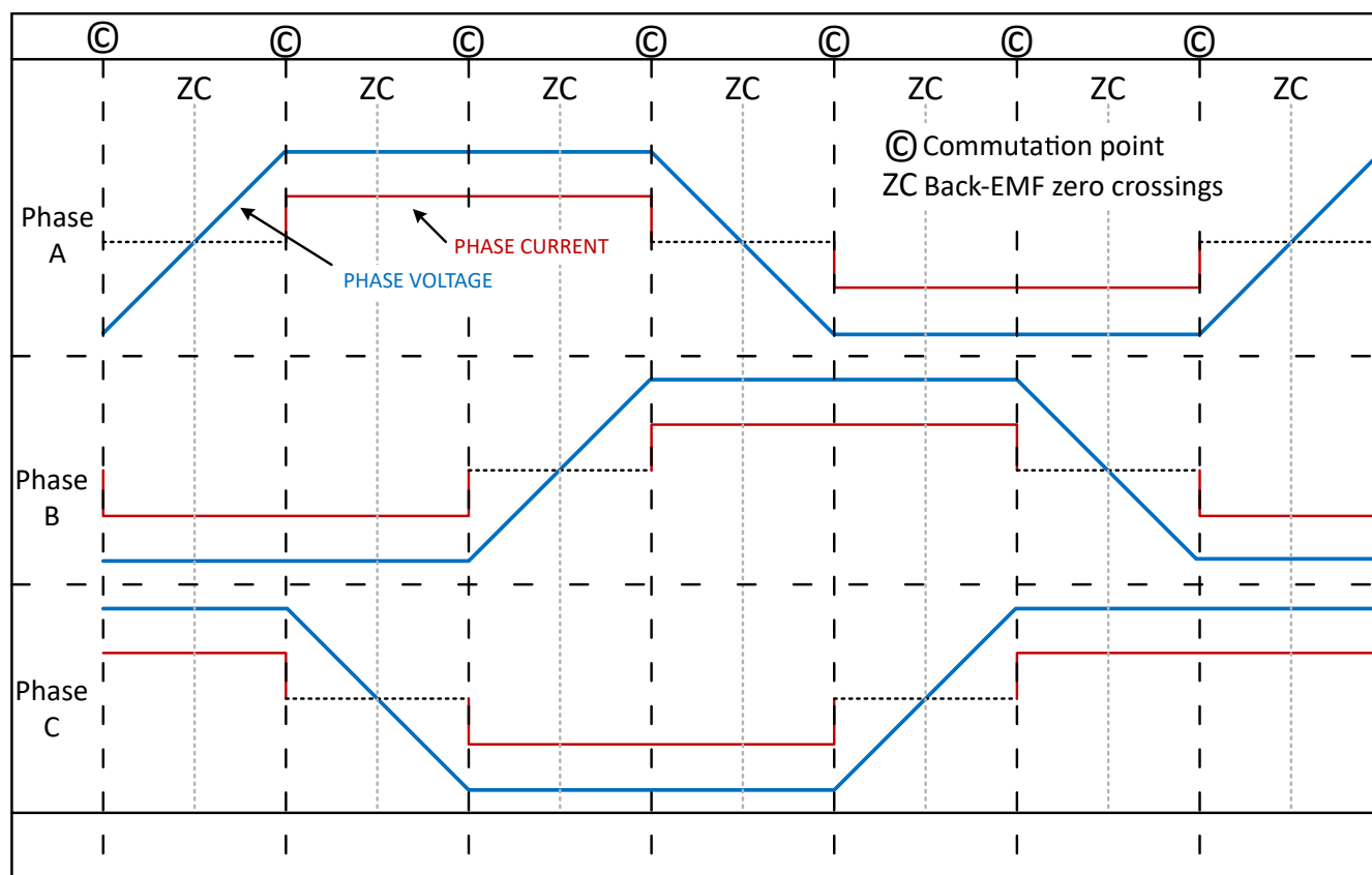
FIG 7-27. 120° commutation
