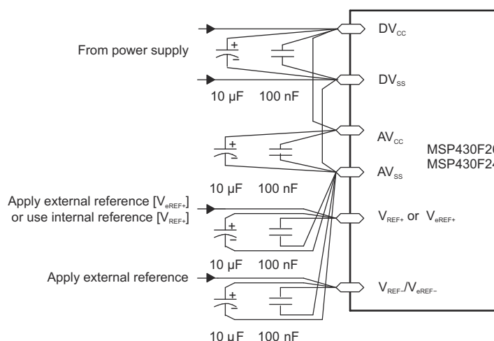
8-39. Supply Voltage and Reference Voltage Design V_{REF}/V_{eREF-} External Supply
