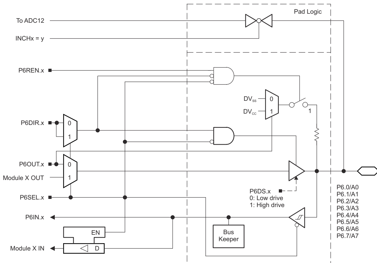
9-10. Port P6 (P6.0 to P6.7) Diagram
