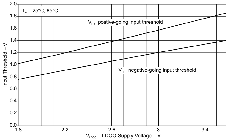
FIG 8-25. Ports PU.0, PU.1 Typical Input Threshold Characteristics
