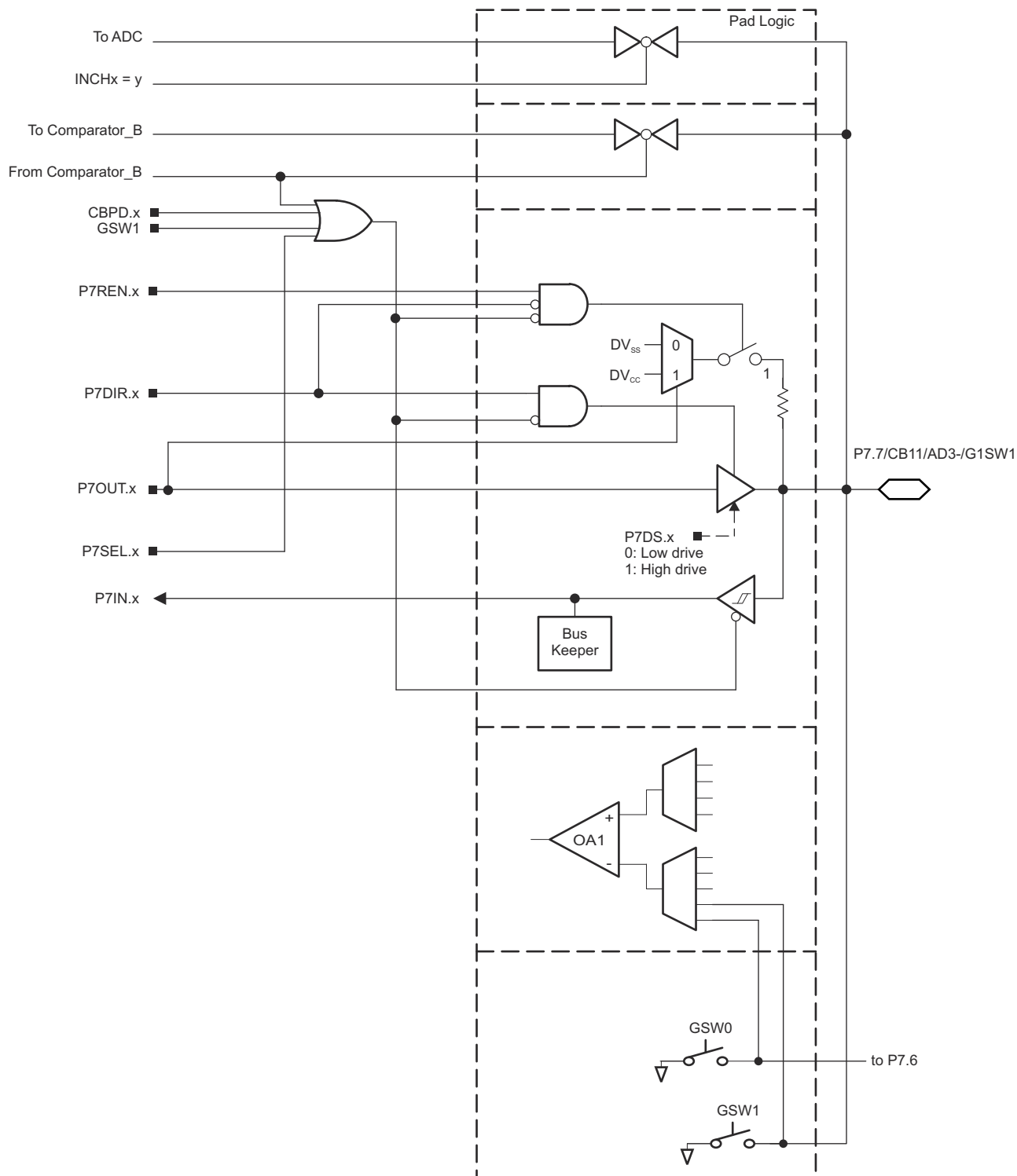
Figure 9-21. Port P7 (P7.7) Diagram
