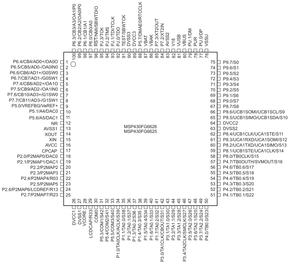
Figure 7-1. 100-Pin PZ Package (Top View), MSP430FG6626IPZ, MSP430FG6625IPZ
