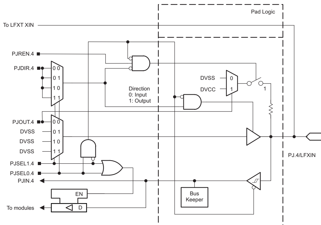
☒ 6-10. Port PJ (PJ.4) Diagram
