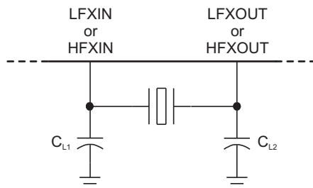
FIG 7-2. Typical Crystal Connection
