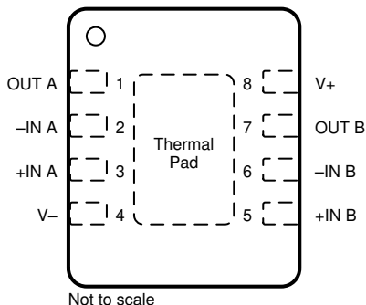
✎ 5-4. OPA1678: DRG Package, 8-Pin SON With Exposed Thermal Pad (Top View)
