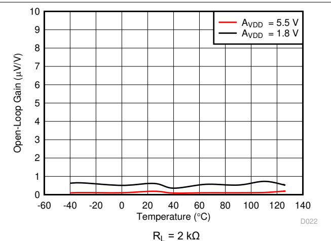
7-22. Open-Loop Gain vs Temperature
