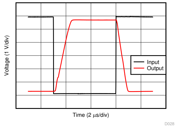
7-30. Overload Recovery
