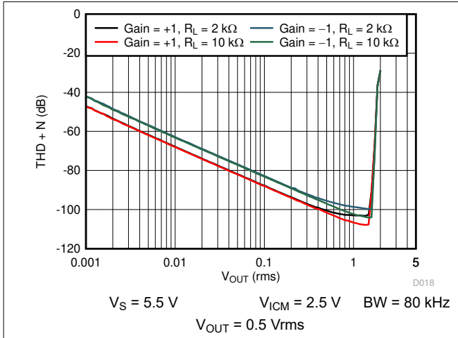
7-19. THD + N vs Amplitude
