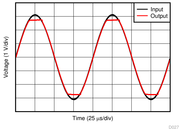
7-29. No Phase Reversal
