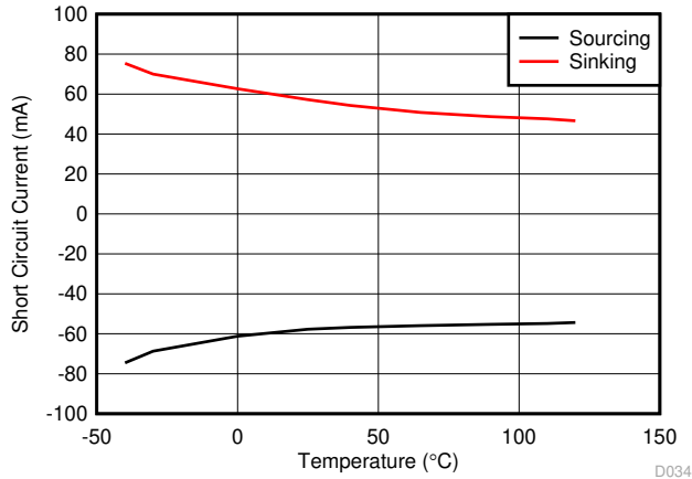
7-35. Short-Circuit Current vs Temperature
