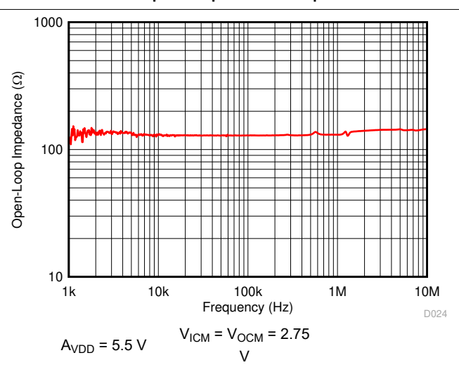
7-24. Open-Loop Output Impedance vs Frequency
