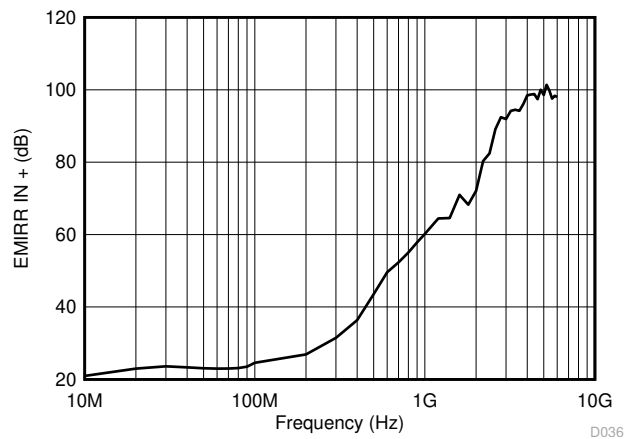
7-37. Electromagnetic Interference Rejection Ratio Referred to Noninverting Input (EMIRR+) vs Frequency
