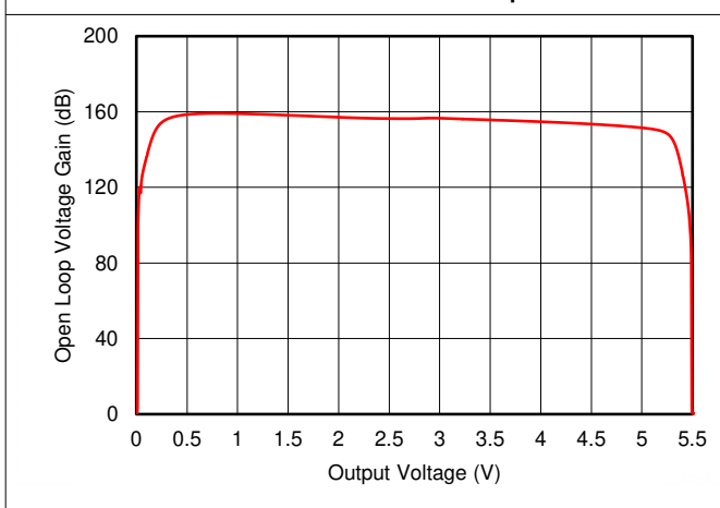
7-23. Open-Loop Gain vs Output Voltage
