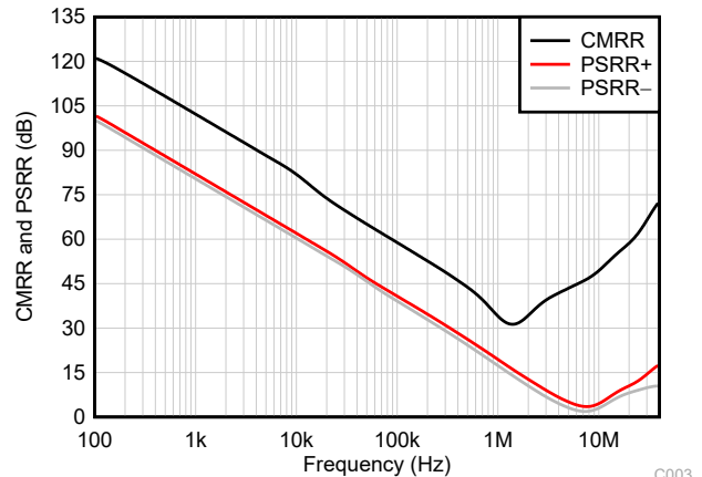
FIG 6-16. CMRR and PSRR vs Frequency
