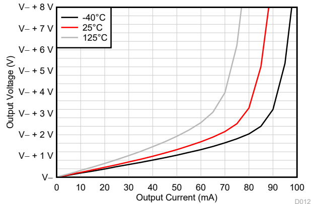
FIG 6-15. Output Voltage Swing vs Output Current (Sinking)
