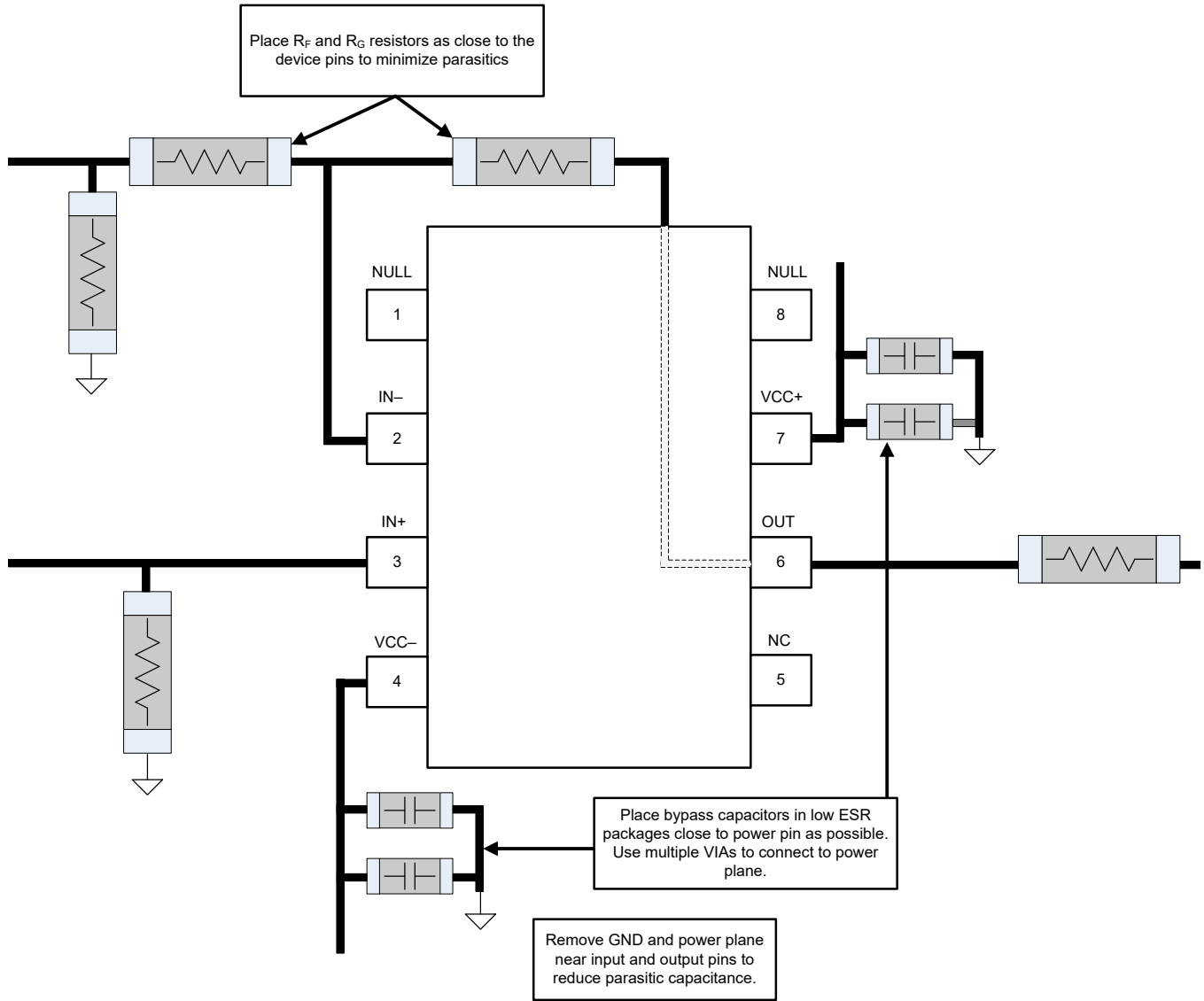
図 7-8. Layout Recommendations
