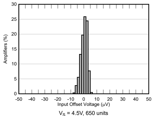
Figure 5-65. Guard Buffer Offset Distribution
