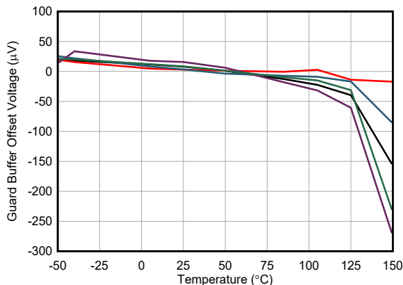
図 5-70. Guard Buffer Offset Drift Distribution
