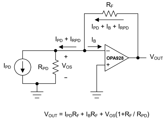
図 7-12. Transimpedance Amplifier DC Model
