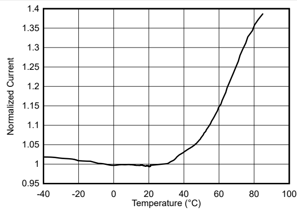
7-11. Standby Current vs Temperature
