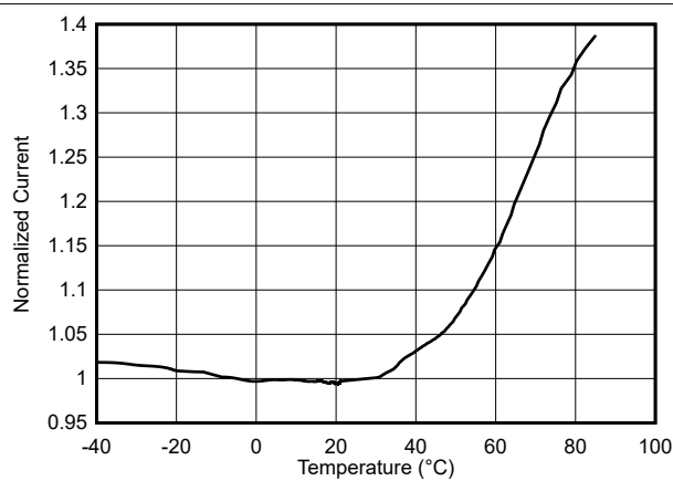
FIG 7-11. Standby Current vs Temperature
