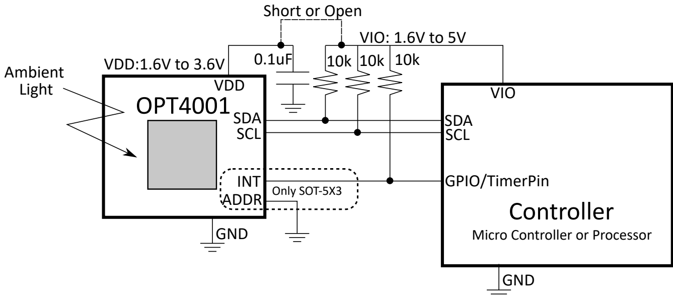
図 9-1. Typical Application Schematic
