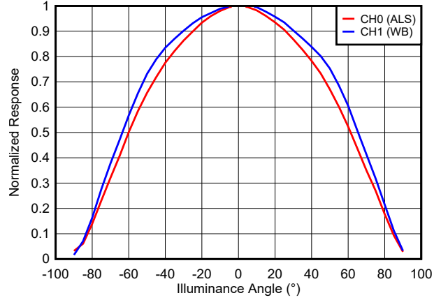
Figure 5-3. Device Response vs Illuminance Angle
