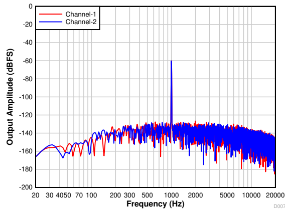
7-19. PCM1821: FFT With a -60\text{-dBr} Input
