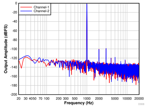
7-20. PCM1821: FFT With a -1\text{-dBr} Input
