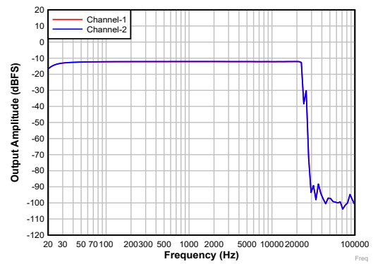
7-6. Differential Input: Frequency Response With a -12-dBr Input
