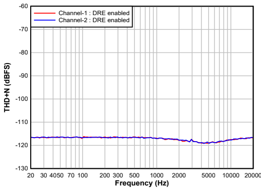
7-3. Differential Input: DR vs Input Frequency With DRE Enabled
