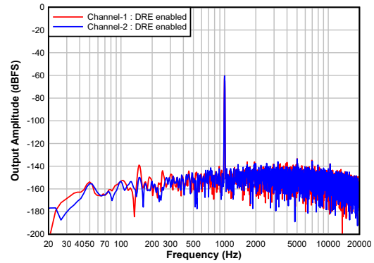
7-20. Single-ended Input: FFT With a -60\text{-dBr} Input and DRE Enabled
