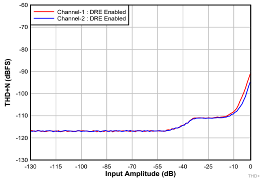
7-1. Differential Input: THD+N vs Input Amplitude With DRE Enabled
