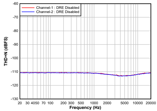
7-4. Differential Input: DR vs Input Frequency With DRE Disabled
