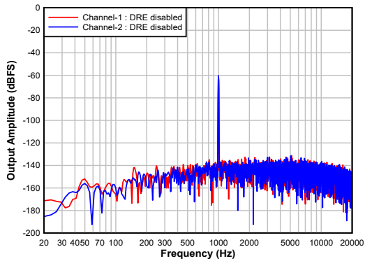
7-21. Single-ended Input: FFT With a -60\text{-dBr} Input and DRE Disabled
