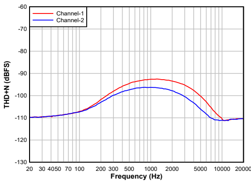
7-5. Differential Input: THD+N vs Input Frequency With a -1-dBr Input
