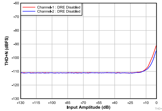
7-2. Differential Input: THD+N vs Input Amplitude With DRE Disabled
