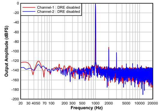
7-22. Single-ended Input: FFT With a -1\text{-dBr} Input
