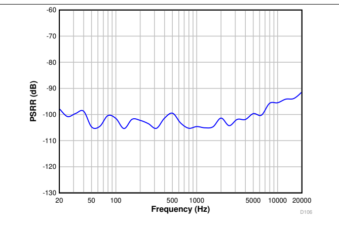
Figure 7. Power-Supply Rejection Ratio vs Ripple Frequency With 100-mV pp Amplitude
