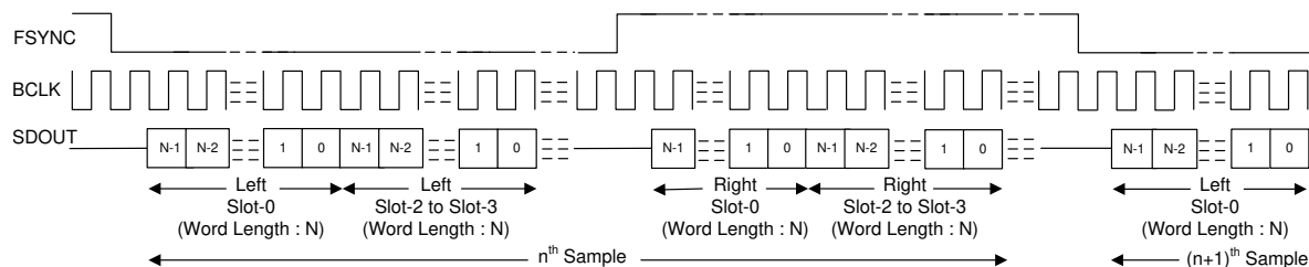
FIG 8-6. I²S Mode Standard Protocol Timing (TX_OFFSET = 0)
