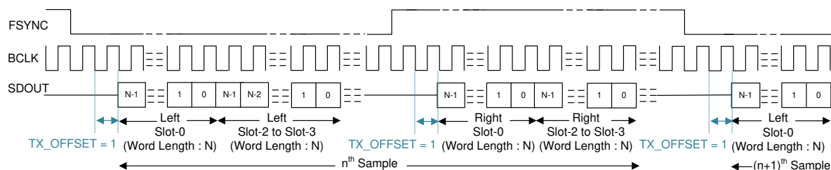
FIG 8-7. I²S Protocol Timing (TX_OFFSET = 1)
