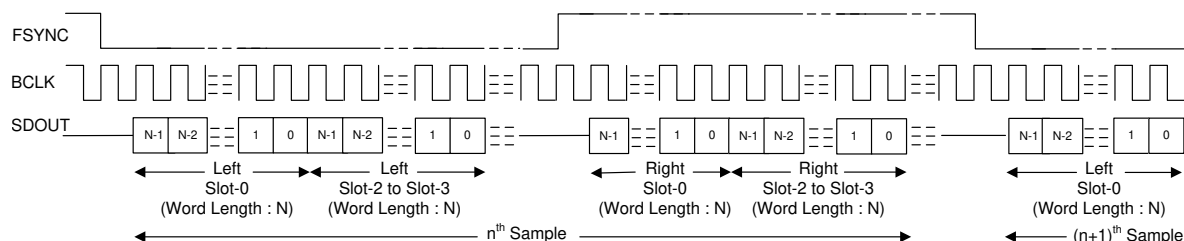
FIG 8-9. I²S Protocol Timing (TX_OFFSET = 0 and BCLK_POL = 1)
