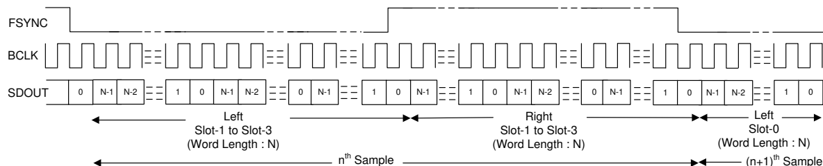
FIG 8-8. I²S Protocol Timing (No Idle BCLK Cycles, TX_OFFSET = 0)
