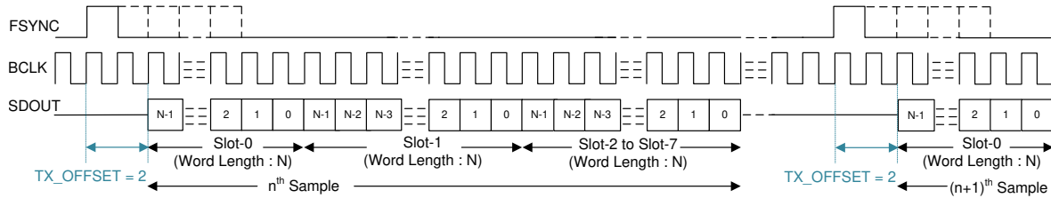
Figure 8-3. TDM Mode Protocol Timing (TX_OFFSET = 2)
