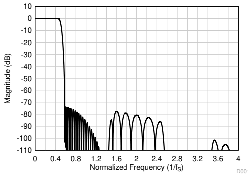
☒ 8-31. Linear Phase Decimation Filter Magnitude Response
