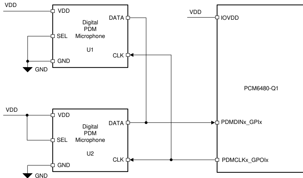
8-19. Digital PDM Microphones Connection Diagram to the PCM6480-Q1
