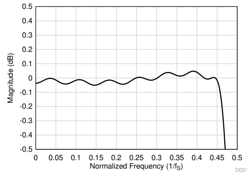
☒ 8-32. Linear Phase Decimation Filter Pass-Band Ripple
