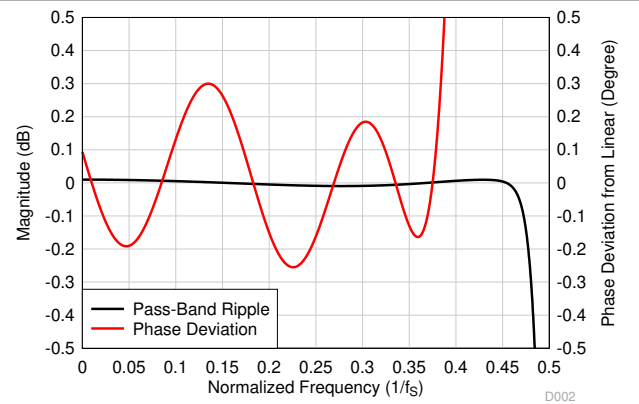
Figure 7-40. Low-Latency Decimation Filter Pass-Band Ripple and Phase Deviation
