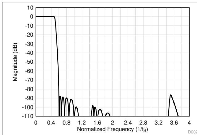
Figure 7-43. Low-Latency Decimation Filter Magnitude Response
