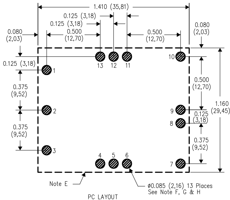
PC LAYOUT
