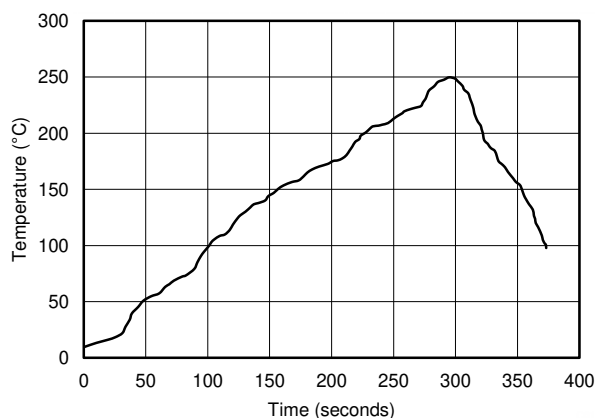
Figure 9-1. Reflow Profile
