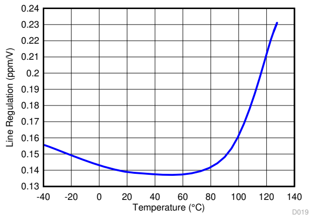
7-6. Line Regulation
