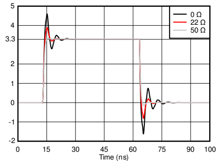
9-2. Typical Application Curve
