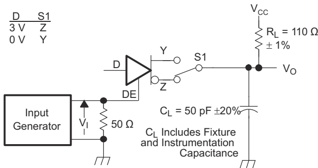
Fig 8-6. Driver High-Level Output Enable and Disable Time Test Circuit and Voltage Waveforms
