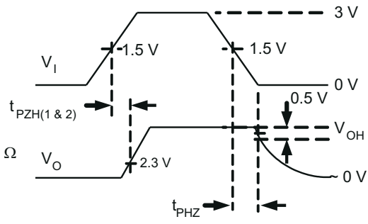
Fig 8-5. Driver Switching Test Circuit and Voltage Waveforms
