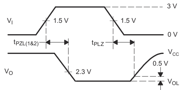
Fig 8-7. Driver Low-Level Output Enable and Disable Time Test Circuit and Voltage Waveforms
