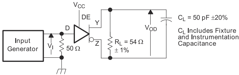
Fig 8-5. Driver Switching Test Circuit and Voltage Waveforms
