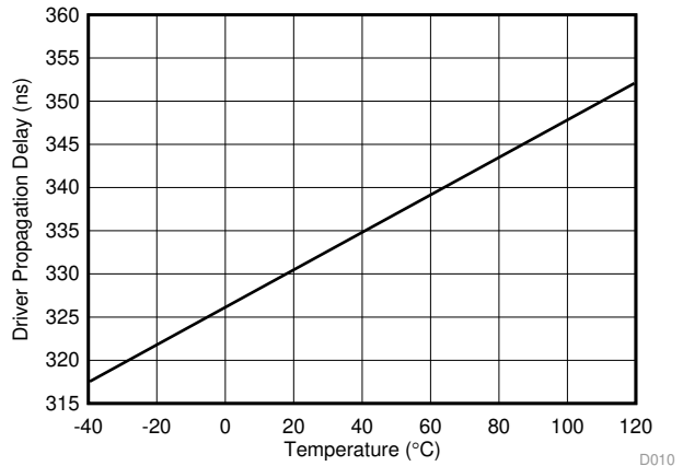
Fig 6. SN65HVD70, SN65HVD71 Driver Propagation Delay vs Temperature
