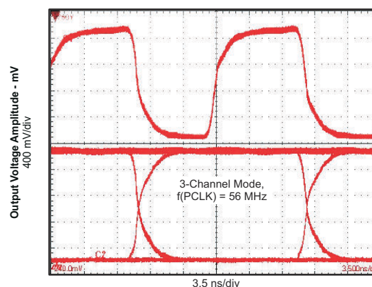
6-13. XGA 3-Channel Output Waveform
