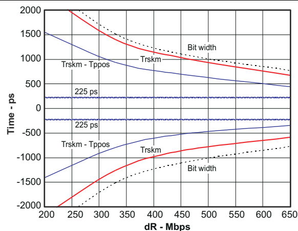
6-11. RSKM, 3-Channel Mode vs Bit Rate
