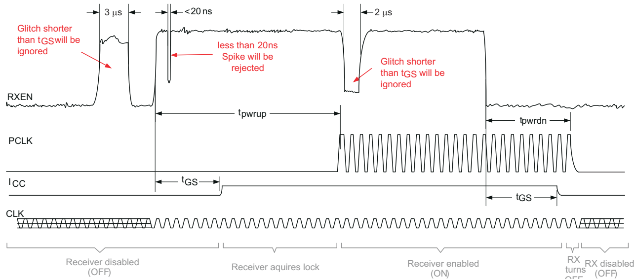
7-10. Receiver Enable and Disable Glitch Suppression Time
