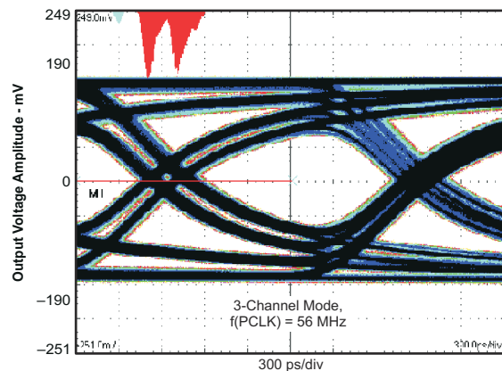
6-12. XGA 3-Channel Output Waveform
