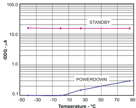
6-2. Quiescent Supply Current vs Temperature
