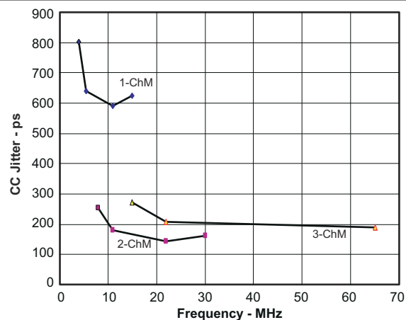
6-8. PCLK Cycle-to-Cycle Output Jitter
