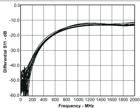
6-15. Input Return Loss
