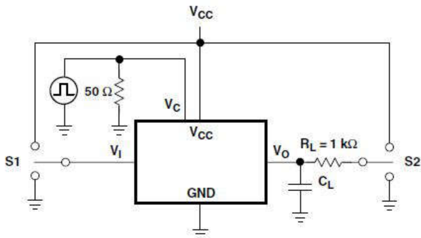
TEST CIRCUIT
