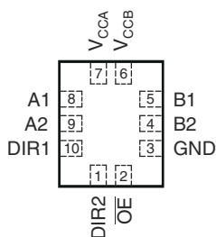
図 4-1. RSW PACKAGE 10-PIN UQFN TOP VIEW
