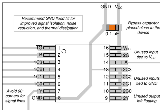
FIG 11-1. Example layout for the SN74HCS153-Q1.
