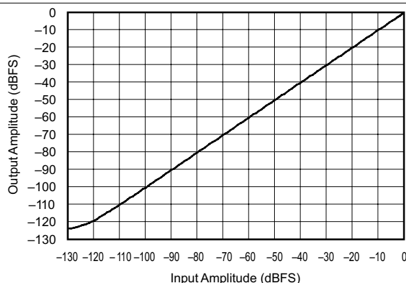
Figure 54. Linearity With f IN = 200 Hz (44.1 kHz:192 kHz)
