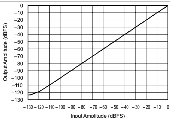
Figure 51. Linearity With f IN = 200 Hz (48 kHz:44.1 kHz)
