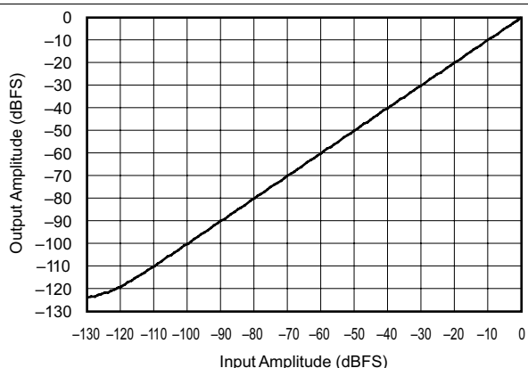
Figure 53. Linearity With f IN = 200 Hz (96 kHz:48 kHz)
