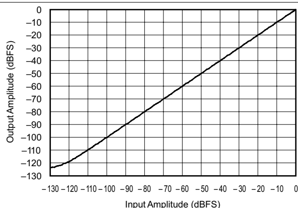
Figure 52. Linearity With f IN = 200 Hz (48 kHz:96 kHz)
