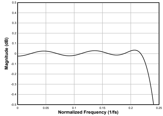
図 6-75. Linear-phase Decimation Filter Pass-Band Ripple
