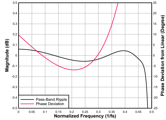
6-99. Ultra Low-latency Decimation Filter Pass-Band Ripple and Phase Deviation
