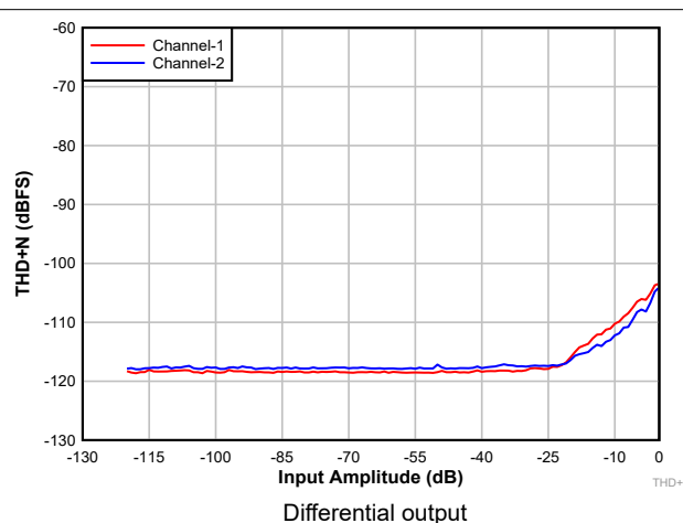
8-3. DAC THD+N Level vs Input
