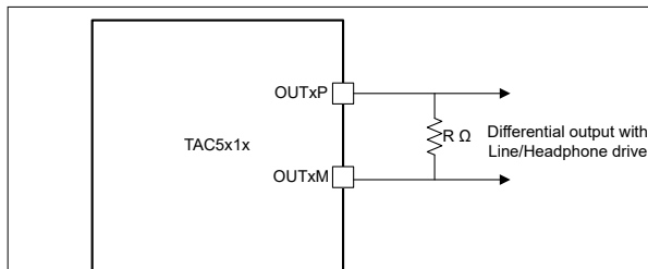
図 6-14. Differential Output Connection (OUT1x_CFG[2:0] = 3'b000)
