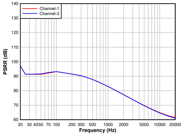
5-19. DAC PSRR vs Frequency
