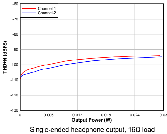
5-9. DAC THD+N Level vs output power
