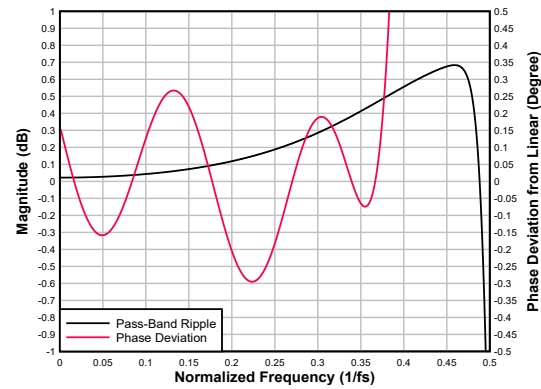
图 6-83. Low-latency Decimation Filter Pass-Band Ripple and Phase Deviation
