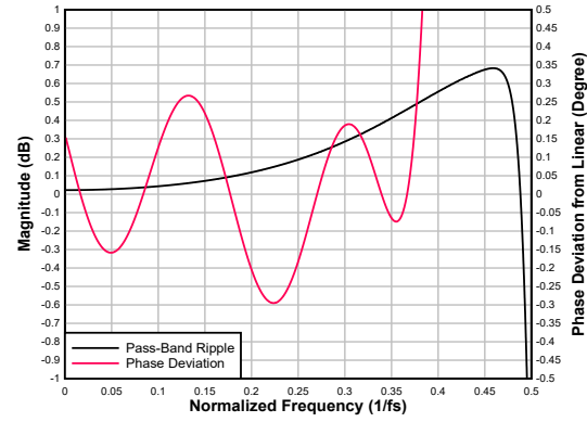
图 6-81. Low-latency Decimation Filter Pass-Band Ripple and Phase Deviation
