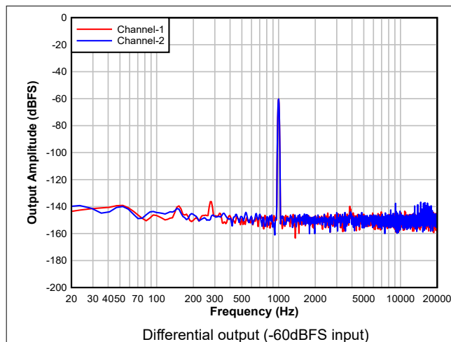
8-2. DAC FFT with -60dBFS Input
