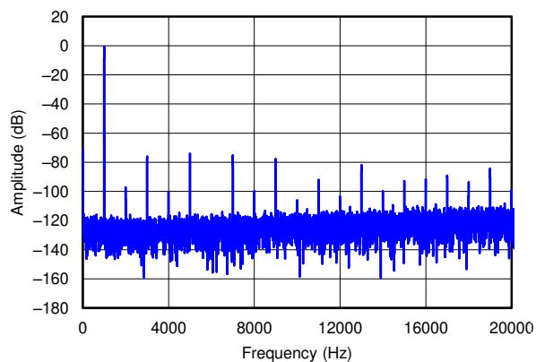
(4Ω Load) 図 5-8. AINL To Speaker FFT Amplitude at 0dBFS vs Frequency
