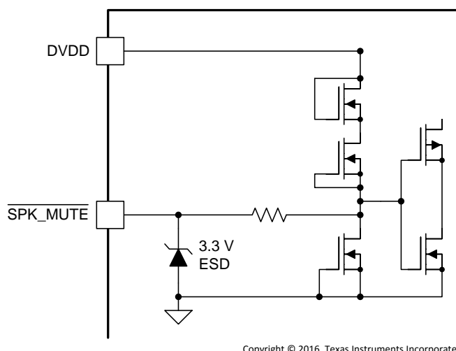
Figure 12. \overline{\text{SPK\_MUTE}} Pin
